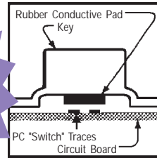
How Conductive Button Shorts Trace
